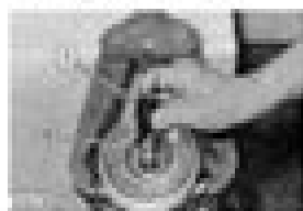
12. Put clean refrigerant oil on shaft seal seal (22). Install shaft seal seal (22) with Tool (23).
