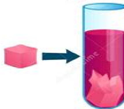
Supersaturated Solution
