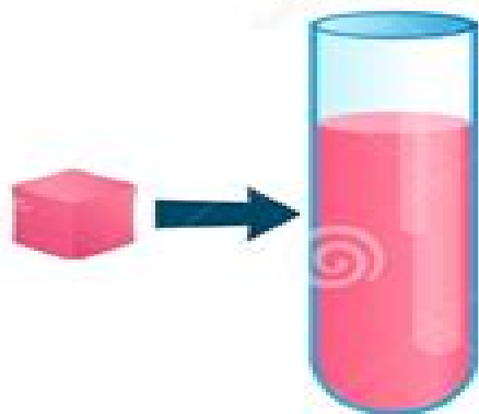
Unsaturated Solution
