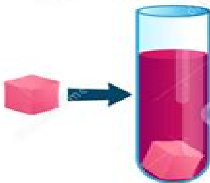
Saturated Solution
