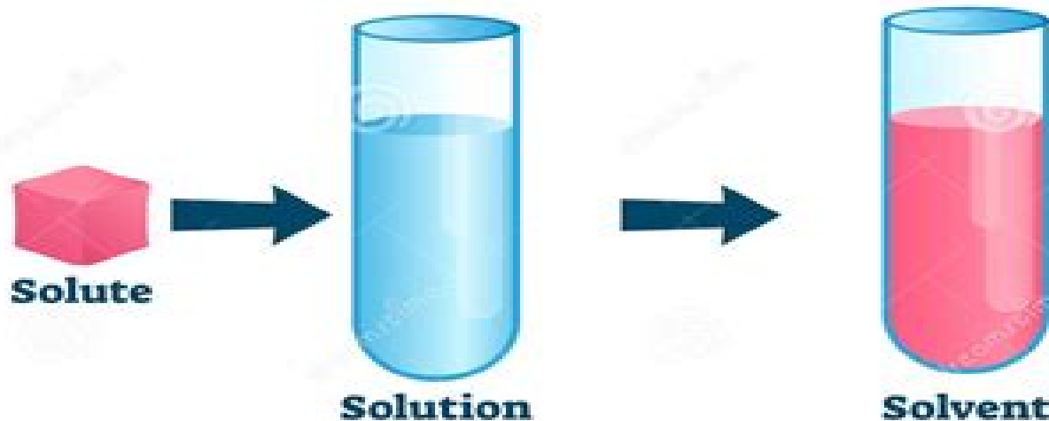
Unsaturated Solution
