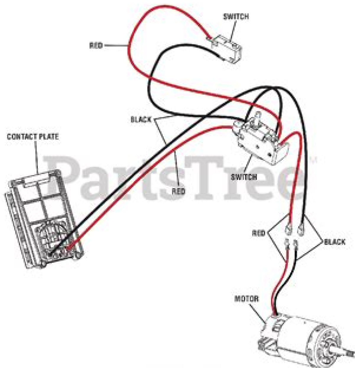
WIRING DIAGRAM
