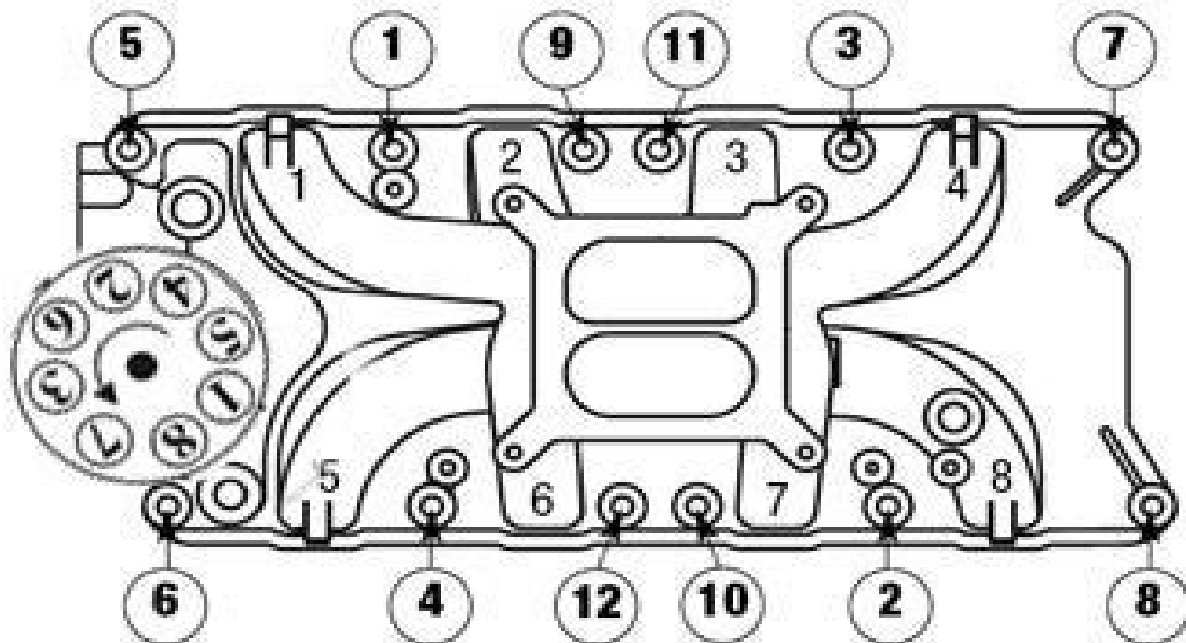
Figure 2 - 260-289-302 Ford Torque Sequence Torque Bolts to 18-20 ft/lbs.
