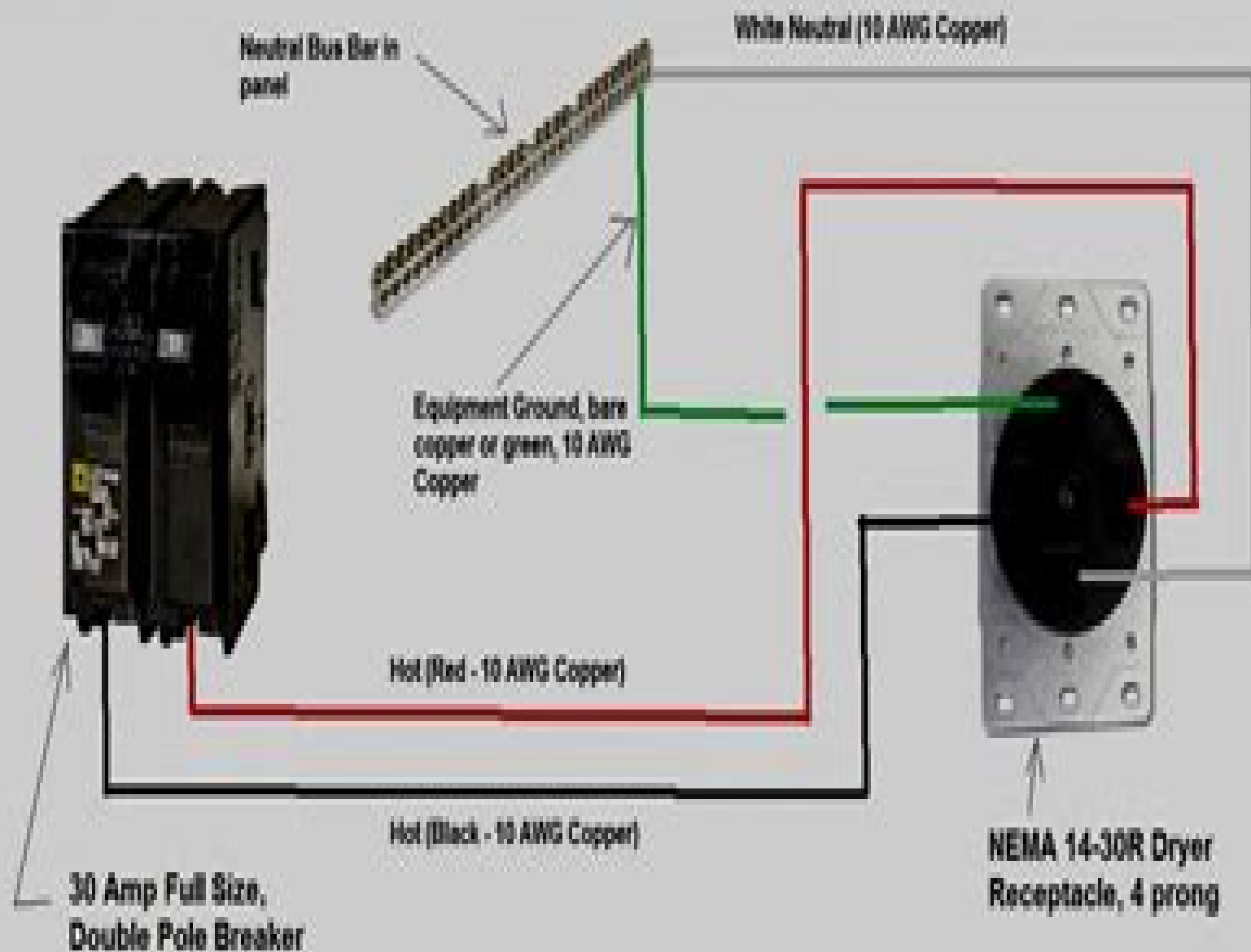
30 Amp, 4 wire, Dryer Circuit with ground
