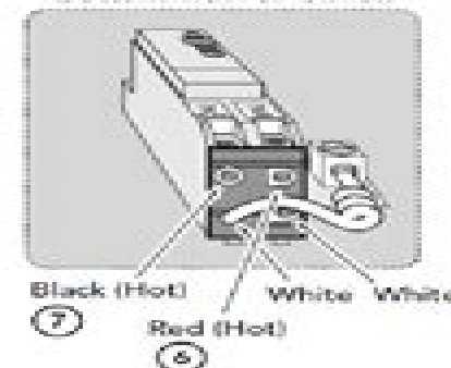
Bottom view of G.F.C.I
