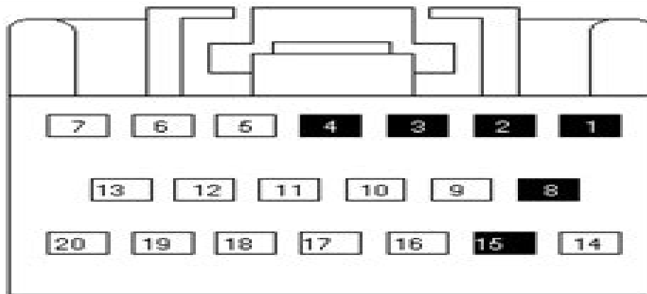
C261 RADIO
