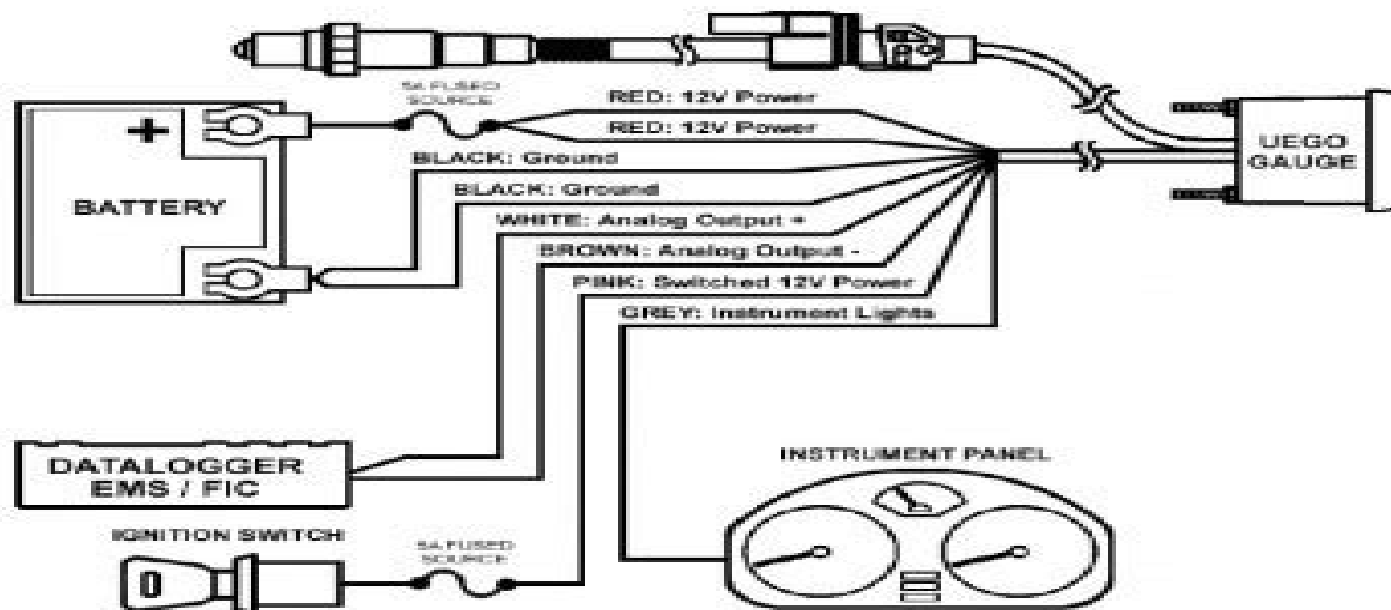
Figure 1. Wiring Schematic
