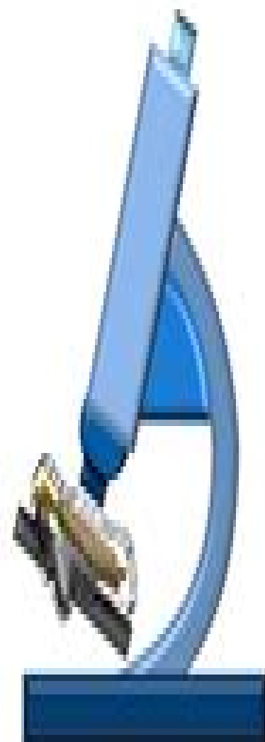
Confocal imaging
