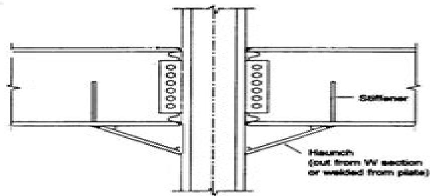
Fig. 4.3.3.3 Welded Haunch Connection
