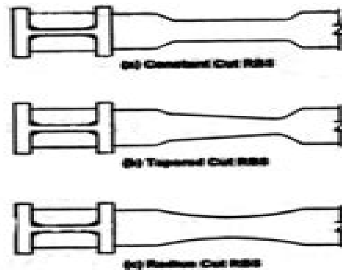
Fig. 4.3.3.2 Contour Detail for RBS Connection
