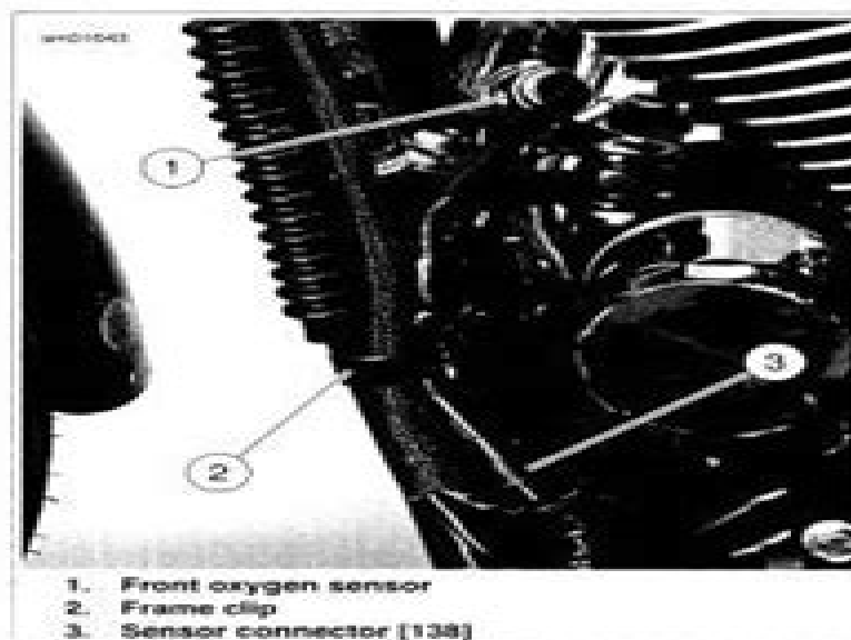
Figure 4-67. Front Oxygen Sensor and Connector, typical (XL model shown)
