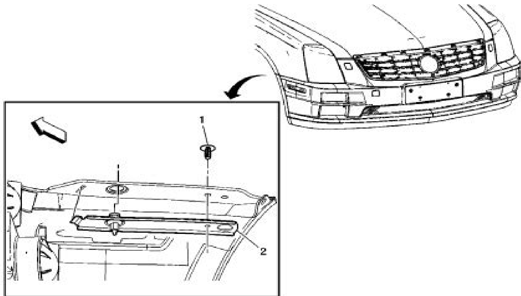
Fig. 5: Identifying Front Bumper Fascia Reinforcement Replacement Courtesy of GENERAL MOTORS CORP.
