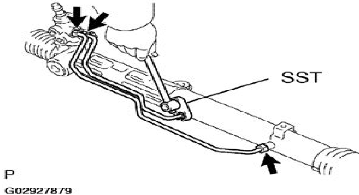
Fig. 5: Removing Turn Pressure Tubes
