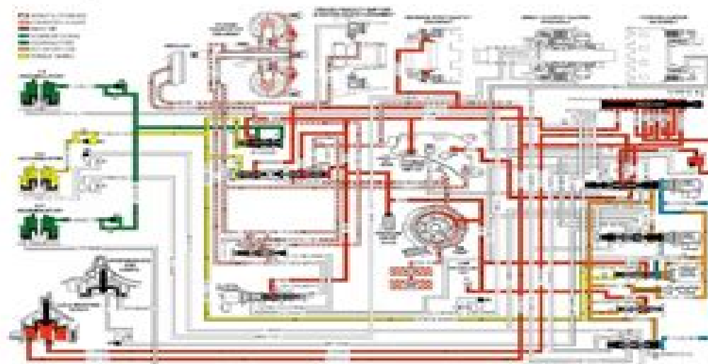
Fig. 5: Reverse (Without Electronic Range Select Mode) Courtesy of GENERAL MOTORS CORP.
