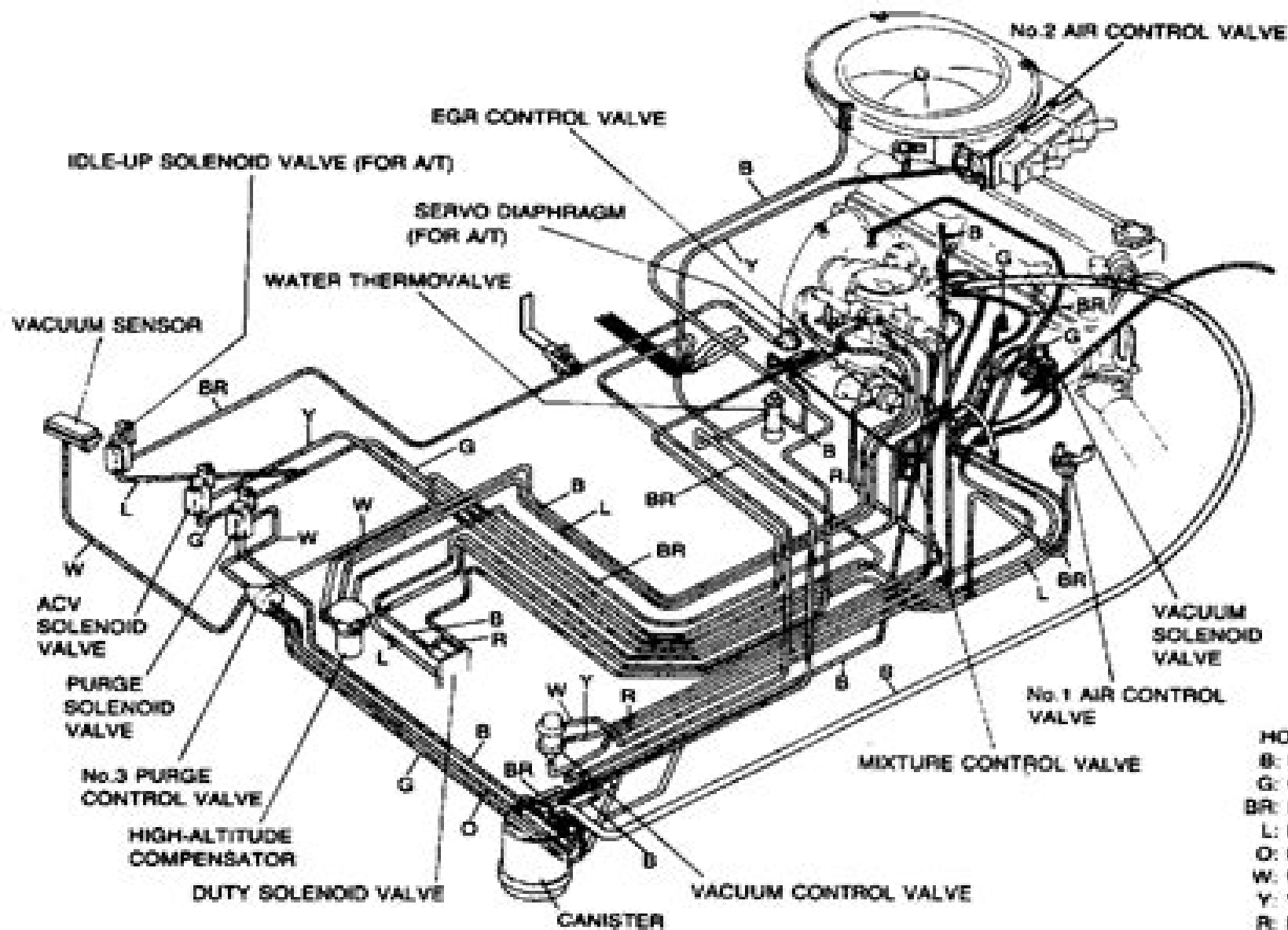
VACUUM HOSE ROUTING DIAGRAM
