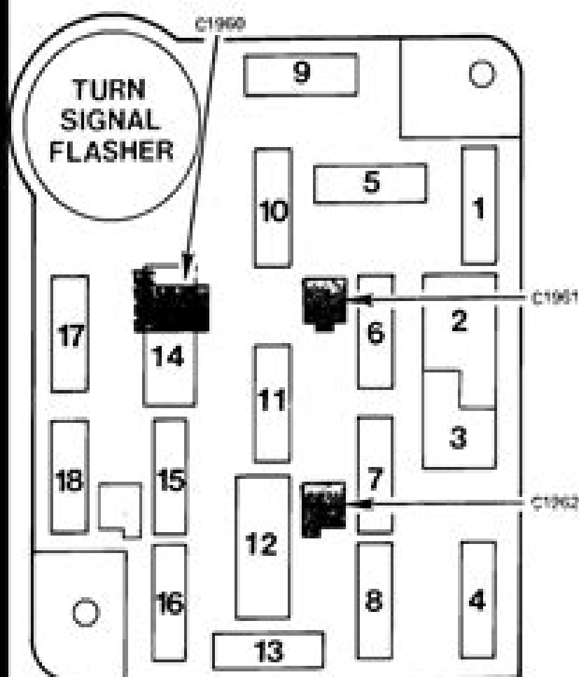
Figure 1 - Fuse Panel
