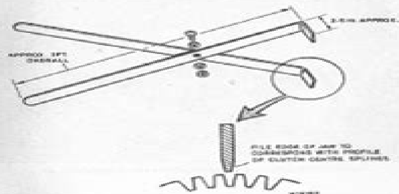
19.9c . . . or you can make your own tool from steel scrap
