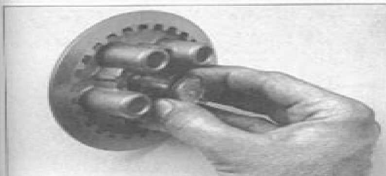
19.7 Remove the pull rod, release bearing and washer from the pressure plate
