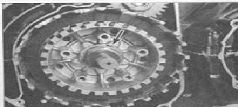
19.9a Bend the tab on the clutch boss lockwasher away from the nut, then remove the nut
