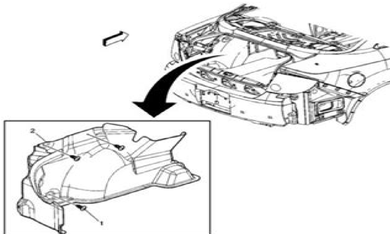
Fig. 19: Identifying Rear Compartment Trim Panel Courtesy of GENERAL MOTORS CORP.
