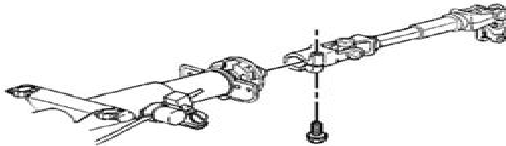
Fig. 5: View Of Upper Pinch Bolt Of Intermediate Steering Shaft Courtesy of GENERAL MOTORS CORP.
