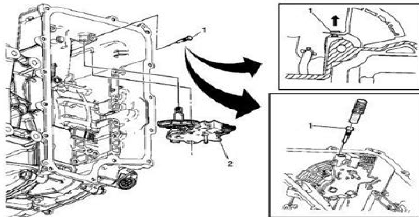
Fig. 1: Manual Shift Detent Lever With Shaft Position Switch Assembly
