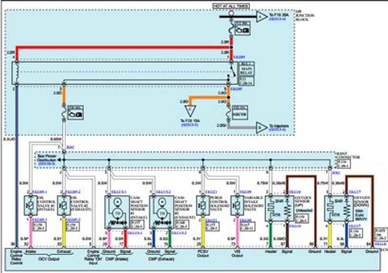
Engine Control System (G4LC : KAPPA 1.4L MPI) (3)
