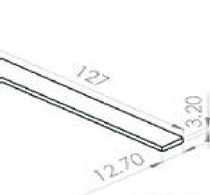
Test specimen as per ASTM D790
