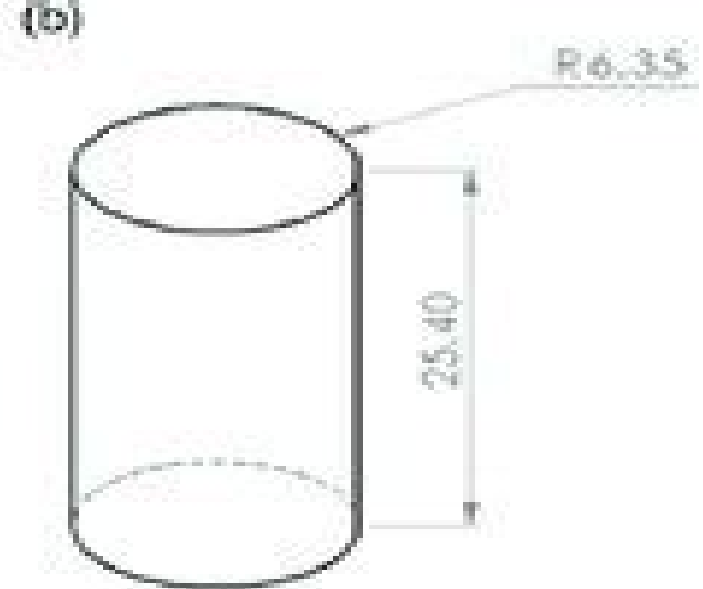
Compressive test specimen as per ASTM D695
