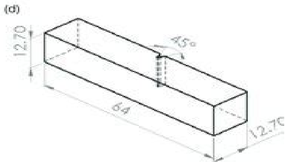
Izod Impact test specimen as per ASTM D256
