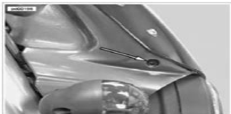
Figure 1-51. Horizontal Headlamp Adjustment Fastener: Lightning
