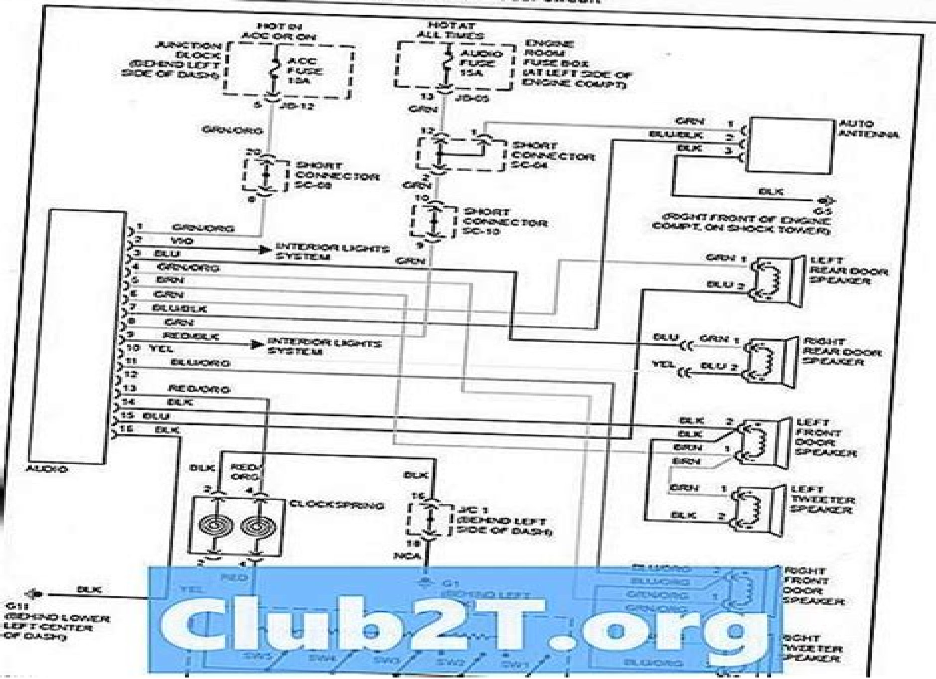
Fig. 38: Base Model Circuit
