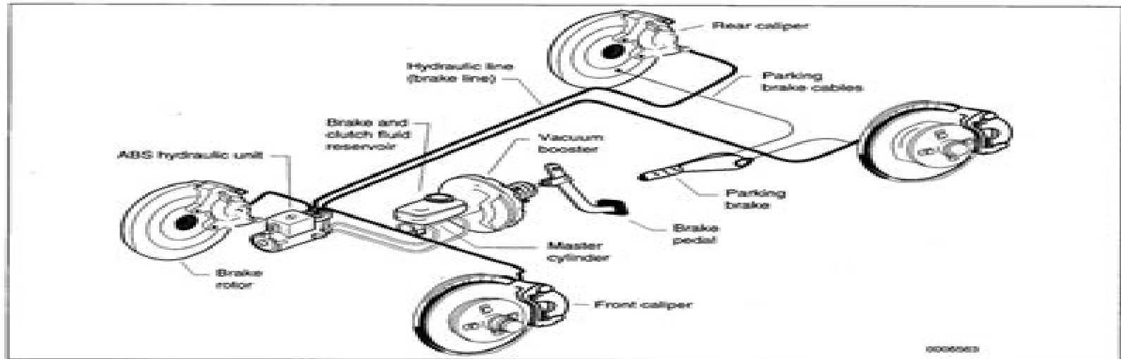
Fig. 3. Schematic view of dual circuit brakes with 4-channel ABS.
