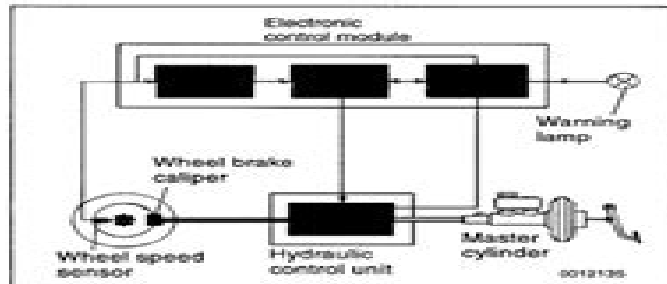
Fig. 4. Schematic representation of ABS.
