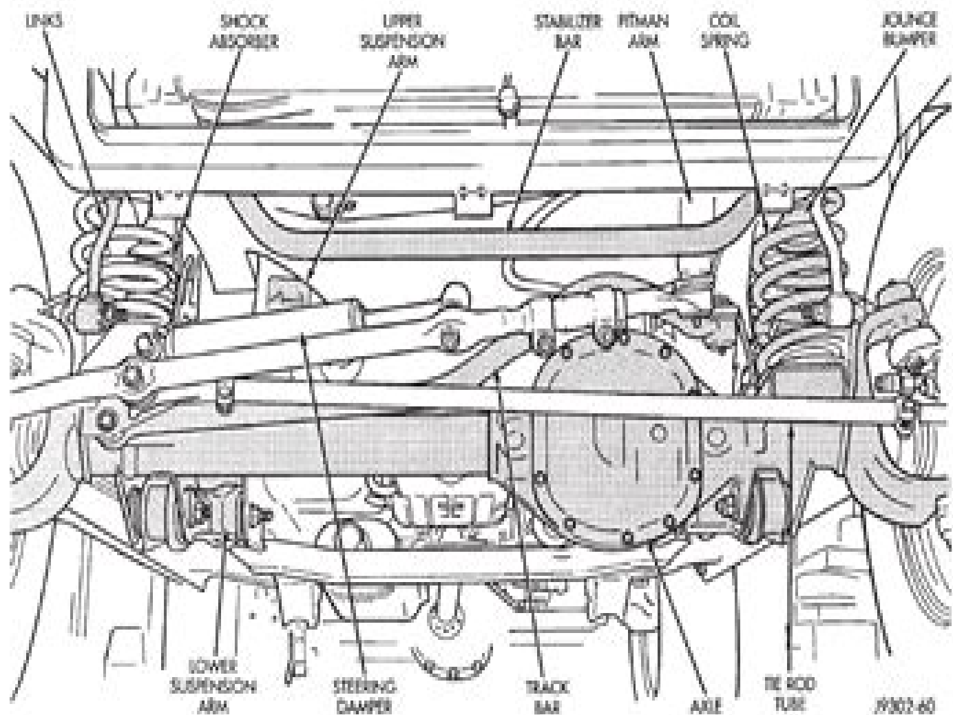
Fig. 1 Front Suspension
