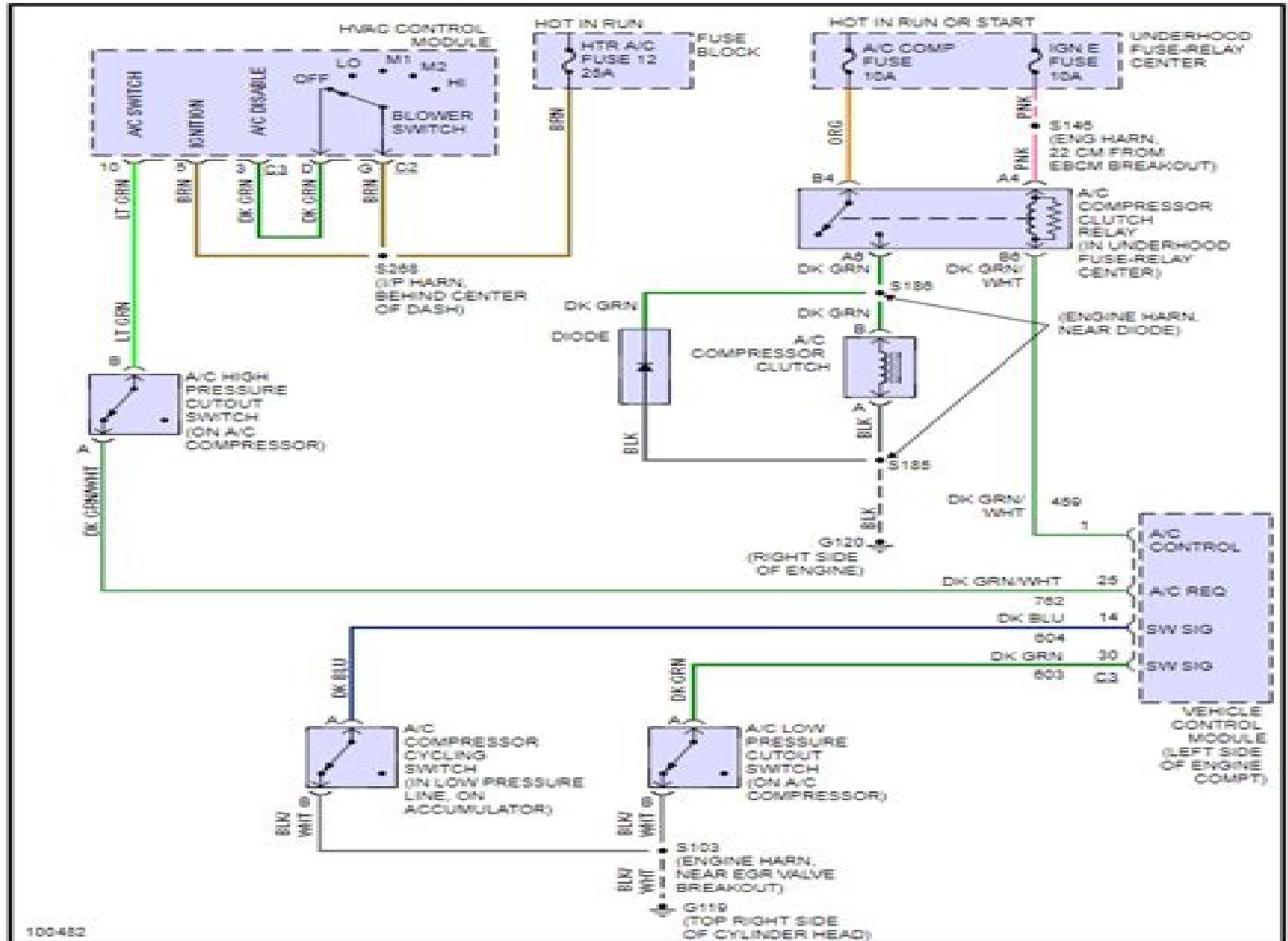
Fig 2: 5.7L (VIN R), Compressor Circuit
