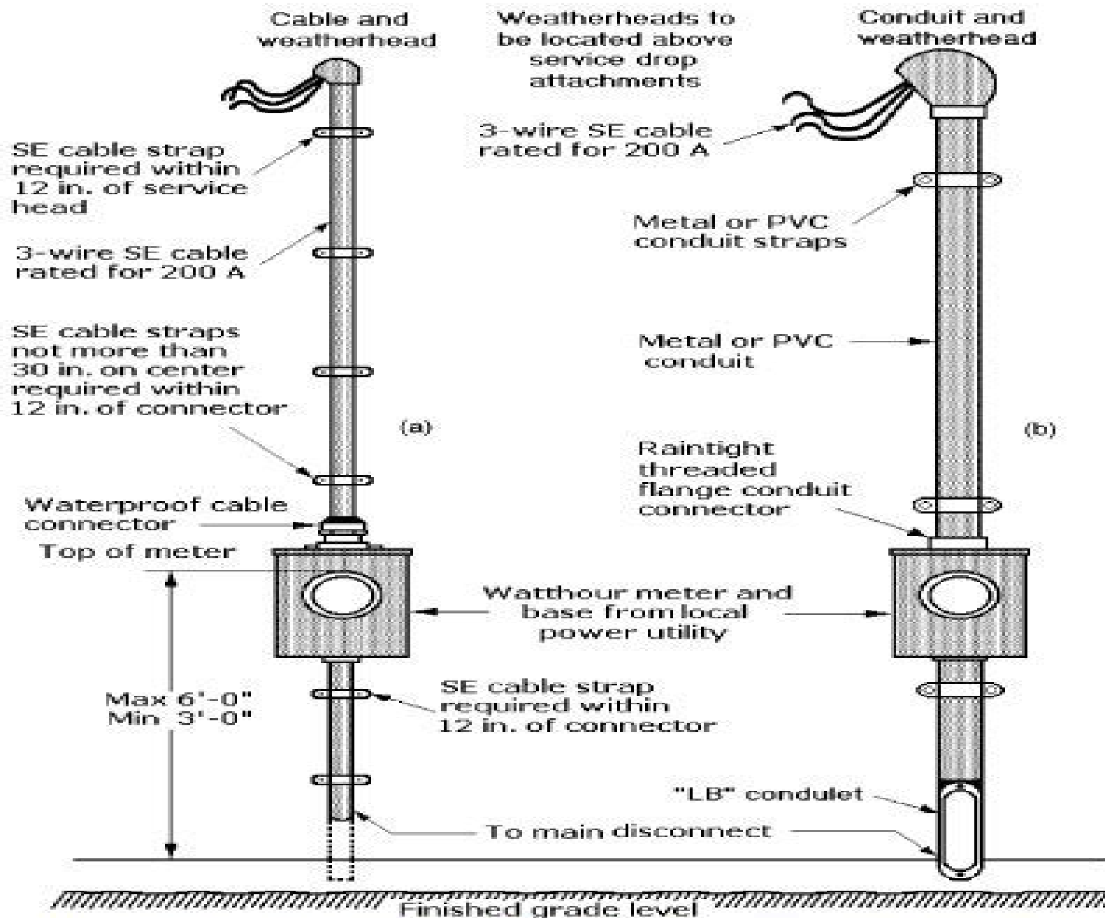
Figure 5-4 Examples of 200-A service entrances using type SE cable: (a) without protective conduit; (b) with conduit.
