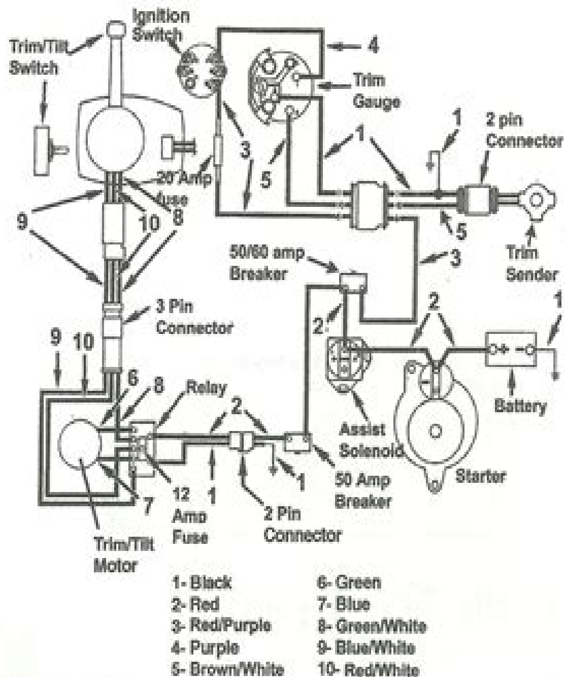
Fig. 102 Power trim/tilt—1993-95 Ford models
