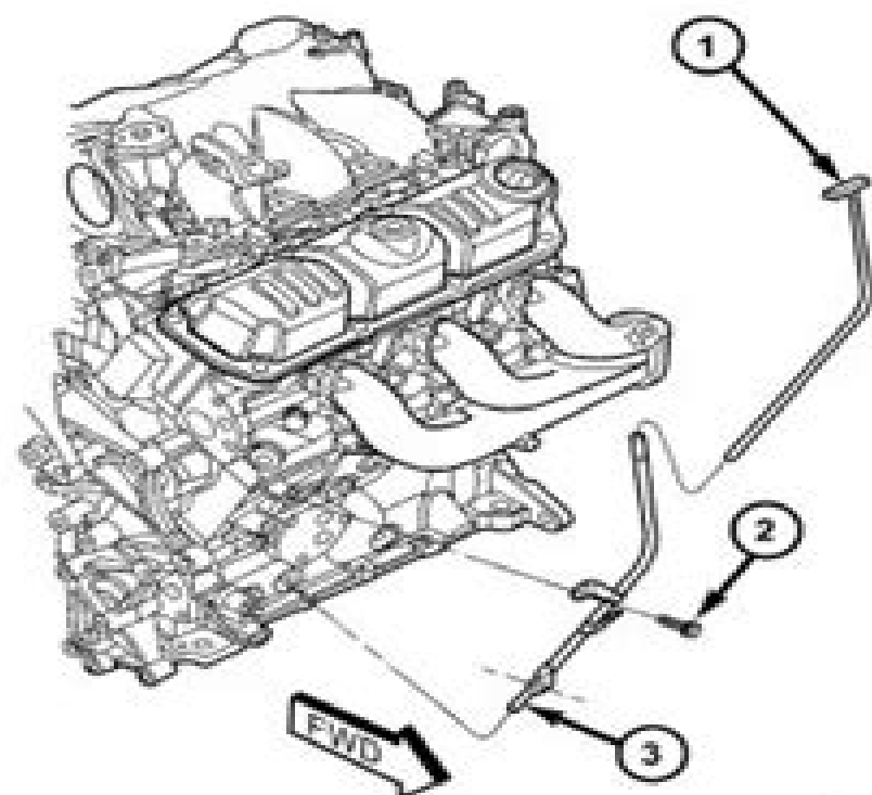
Fig. 18 DIPSTICK &amp; TUBE
